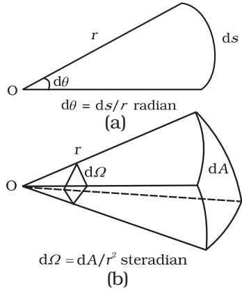
Fig. 2.1 Description of (a) plane angle d\theta and (b) solid angle d\Omega .
