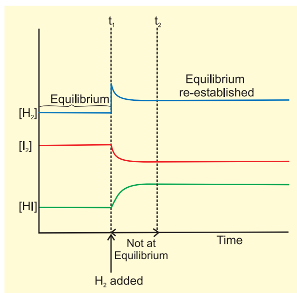
Fig. 7.8 Effect of addition of \text{H}_2 on change of concentration for the reactants and products in the reaction, \text{H}_2(\text{g}) + \text{I}_2(\text{g}) \rightleftharpoons 2\text{HI}(\text{g})
